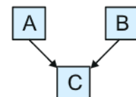
Multiple Inheritance
